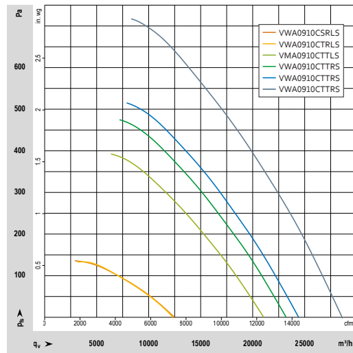
Characteristic curve field for size 910 (measured without fan housing)
