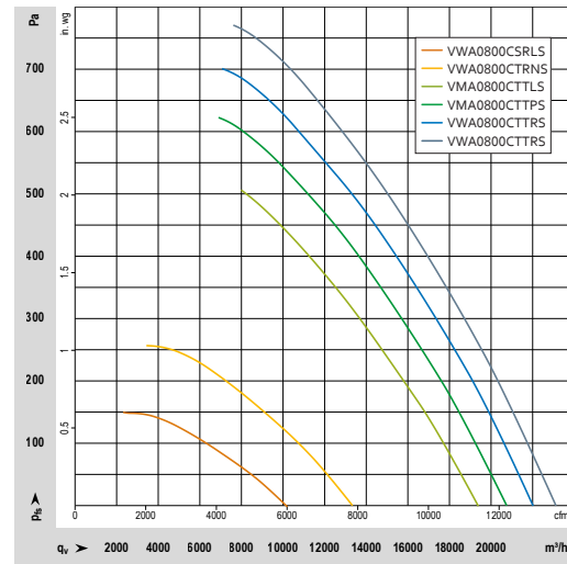
Characteristic curve field for size 800 (measured without fan housing)
