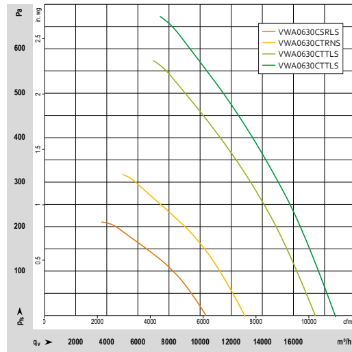
Characteristic curve field for size 630 (measured without fan housing)
